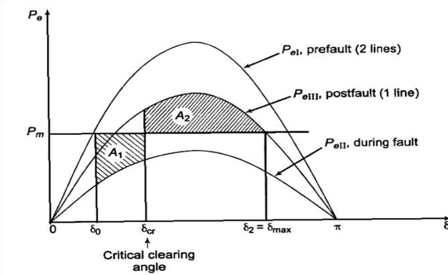
Fig.4.15 Fault on middle of one line of the system of, case of critical clearing angle
