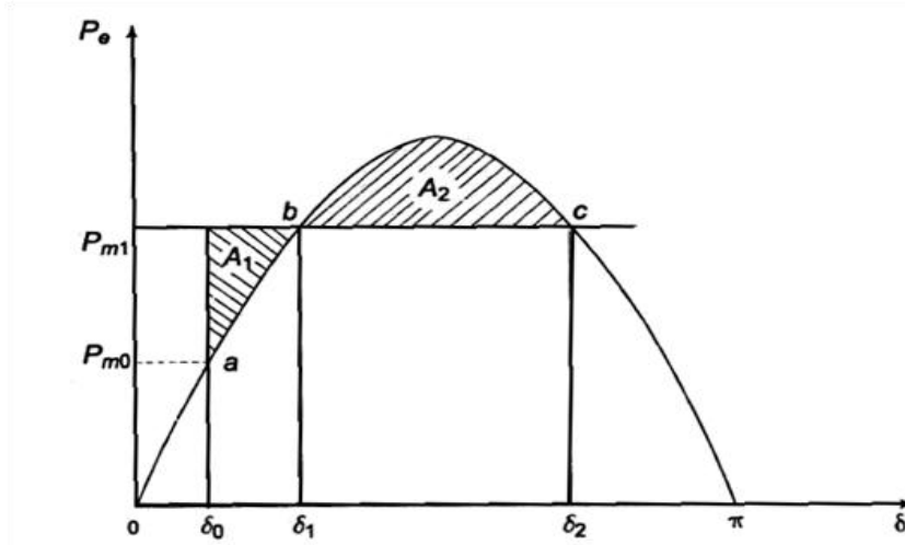
Fig. 4.10 Limiting case of transient stability with mechanical input suddenly increased
